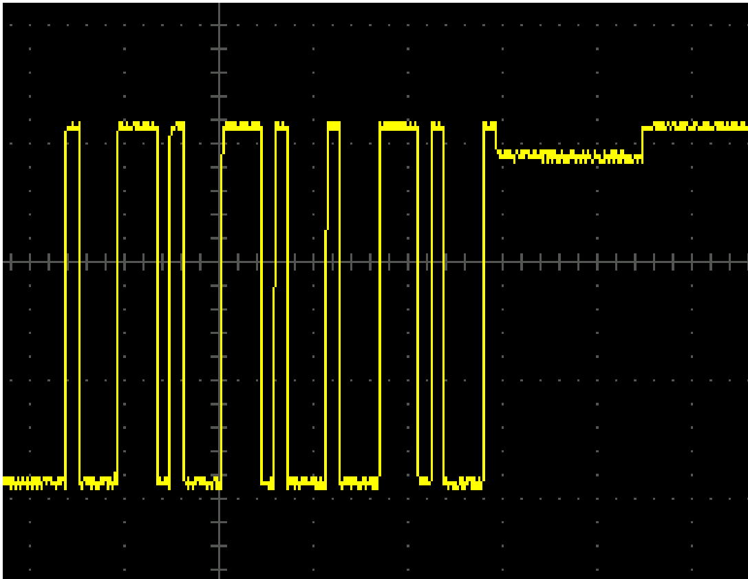
DATA BYTES FROM THE SMART MODULES TO THE MECCABRAIN
