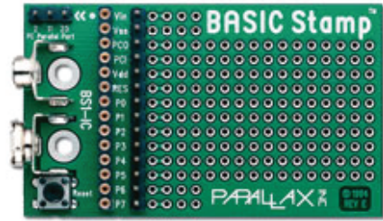
Using Carrier Board for BS1-IC
