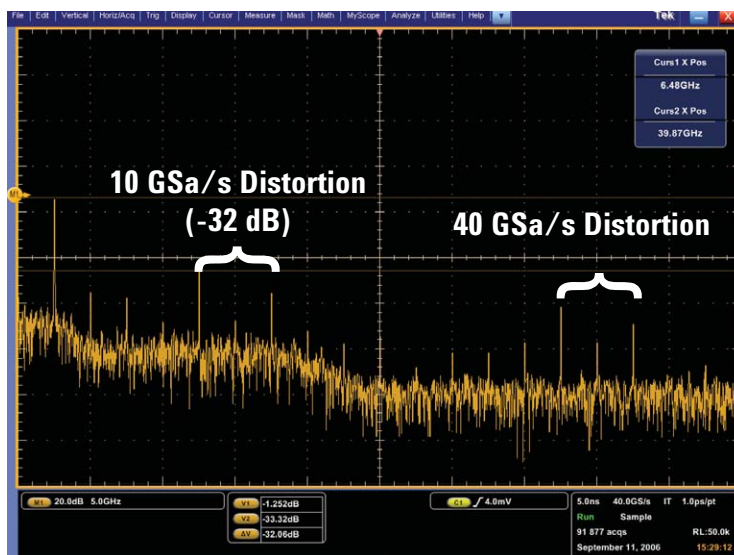
Figure 14b: FFT analysis of 2.5-GHz sine wave captured on a Tektronix DPO7254 sampling at 40 GSa/s
