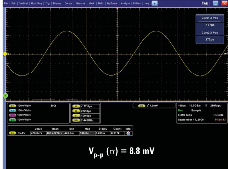
Figure 13a: 2.5-GHz sine wave captured on Tektronix DP07254 2.5-GHz bandwidth oscilloscope sampling at 10 GSa/s (non-interleaved)
