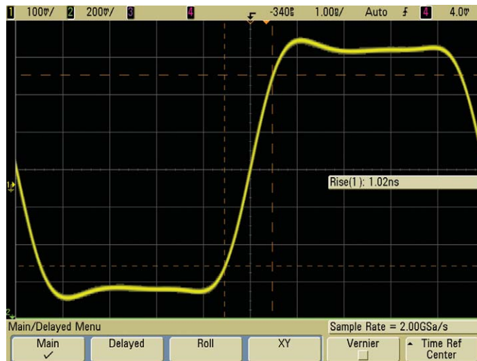
Figure 6: Agilent MSO7054A 500-MHz bandwidth scope sampling at 2 GSa/s shows an accurate measurement of this 100-MHz clock with a 1-ns edge speed
