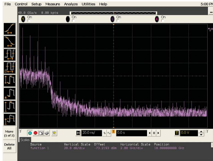
Figure 16a: FFT analysis on 400-MHz clock using an Agilent Infiniium DS080304A 3-GHz bandwidth oscilloscope
