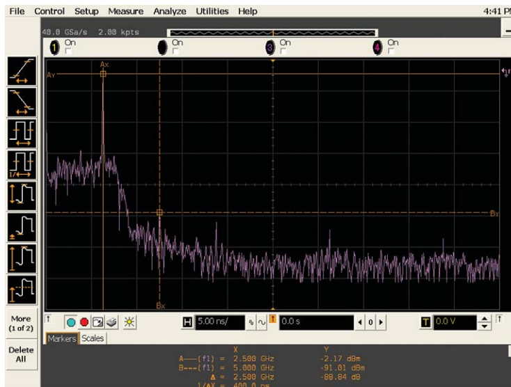
Figure 14a: FFT analysis of 2.5-GHz sine wave captured on an Agilent Infiniium DSO80304A sampling at 40 GSa/s
