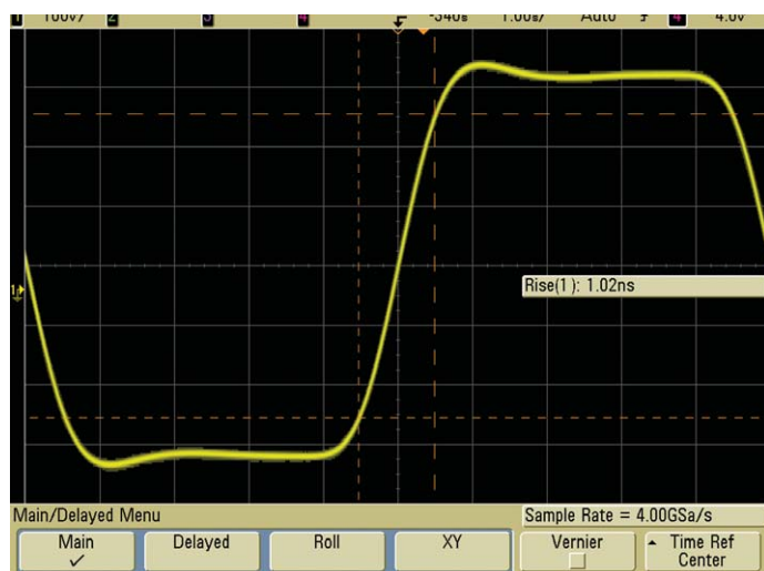
Figure 7: Agilent MSO7054A 500-MHz bandwidth scope sampling at 4 GSa/s produces minimal measurement improvement over sampling at 2 GSa/s
