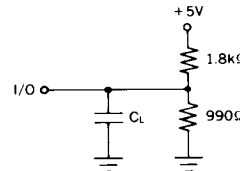
C_L = 5pF (Includes Jig Capacitance)
