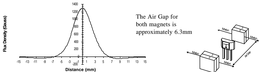
Graph 10, Push-Pull Activation Using Slide-by Method with Magnet A The Push-Push Method
