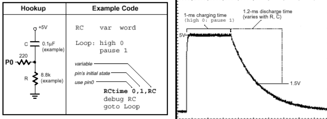
Figures 15.3 and 15.4: Rctime hookup diagram/example code (left) and storage-oscilloscope trace (right)
