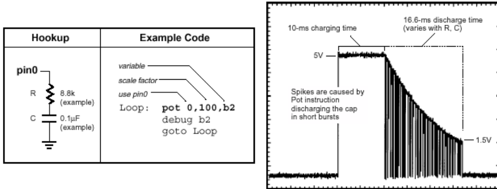
Figures 15.1 and 15.2: Pot hookup diagram/example code (left) and storage-oscilloscope trace (right)
