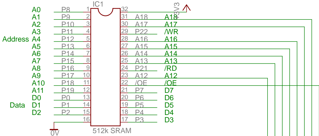
Address A0 to A11 selected from the propeller
