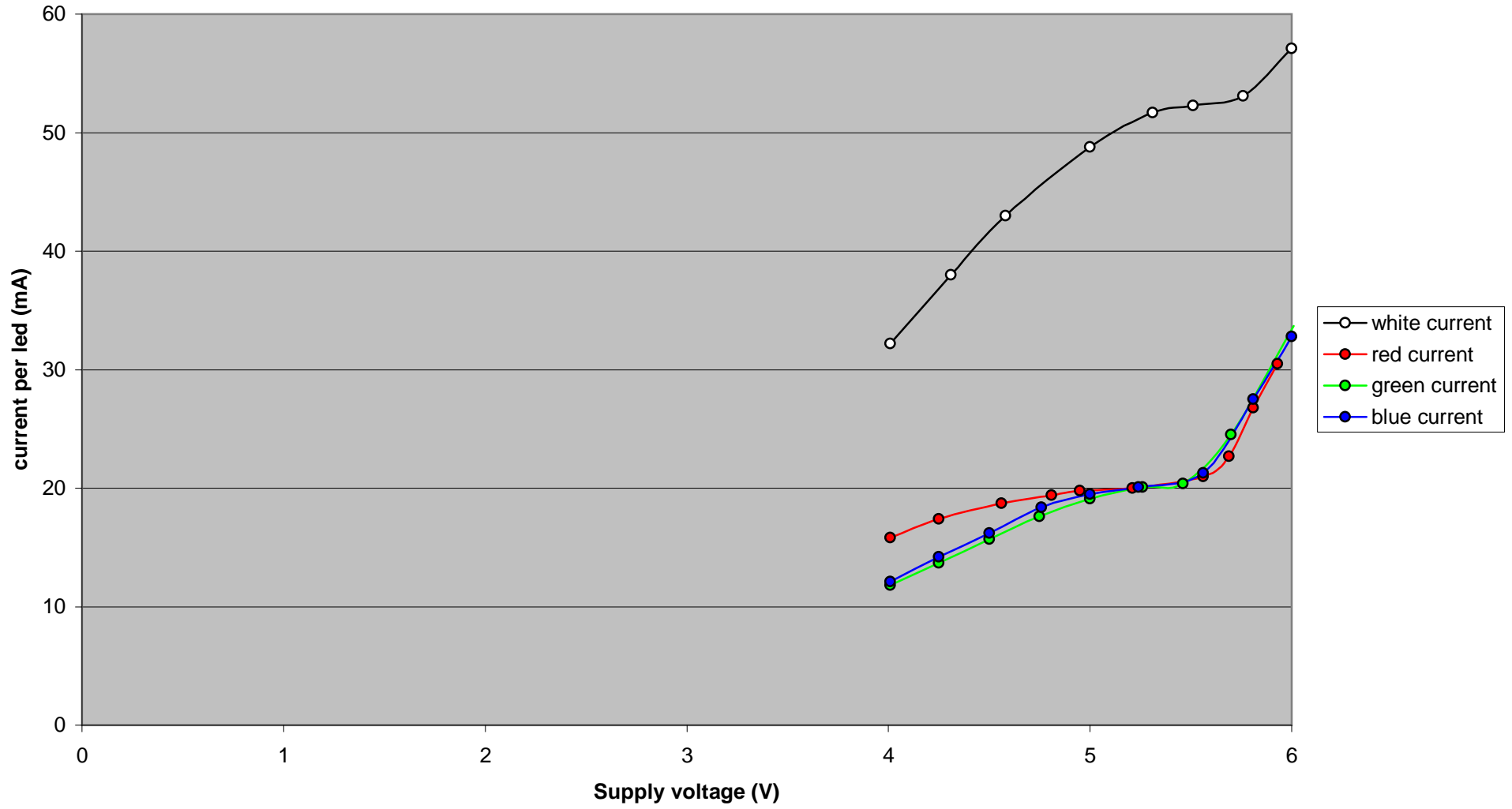
WS2812B characteristic
