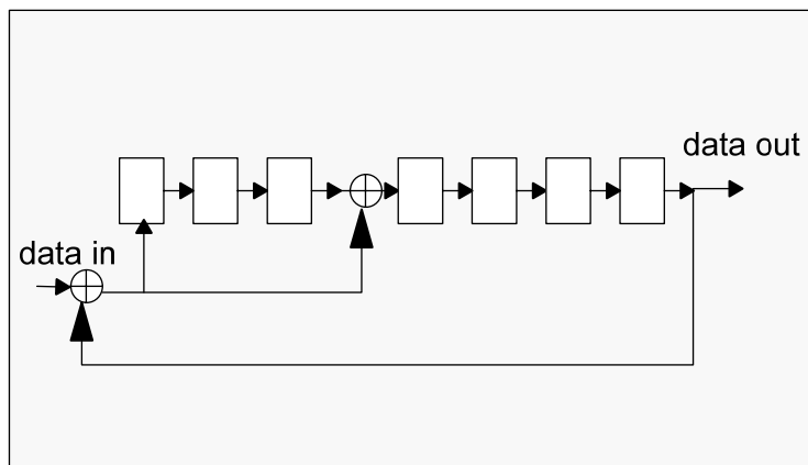
Figure 4-6: CRC7 Generator/Checker
