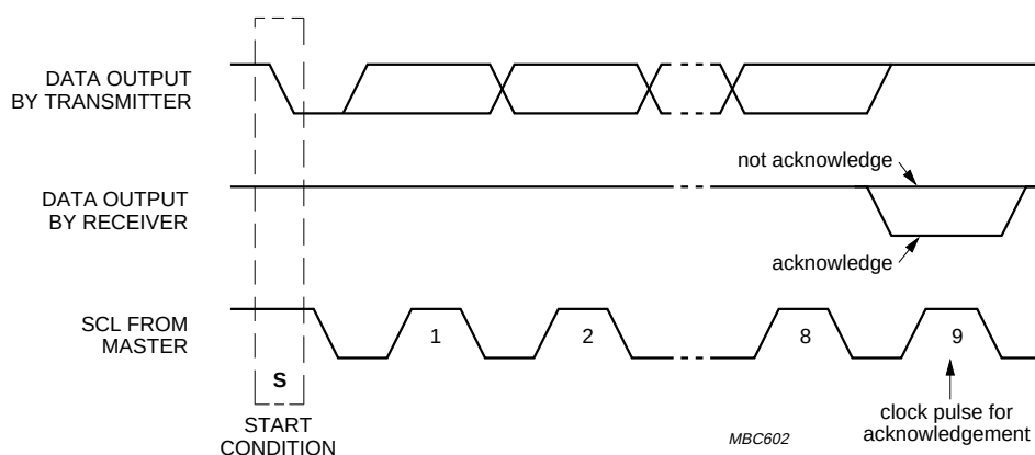
Fig.16 Acknowledgment on the I 2 C-bus.
