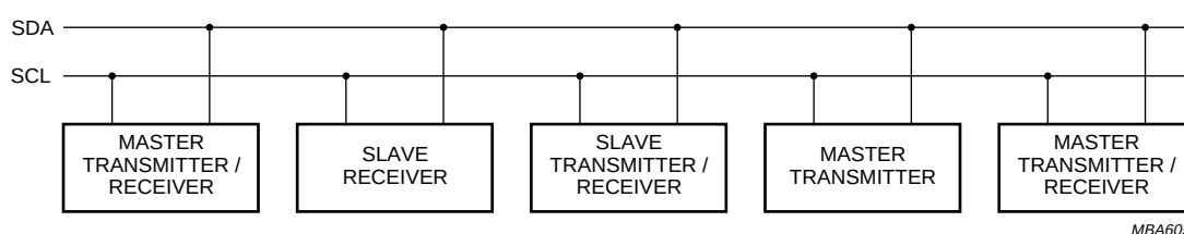
Fig.15 System configuration.
