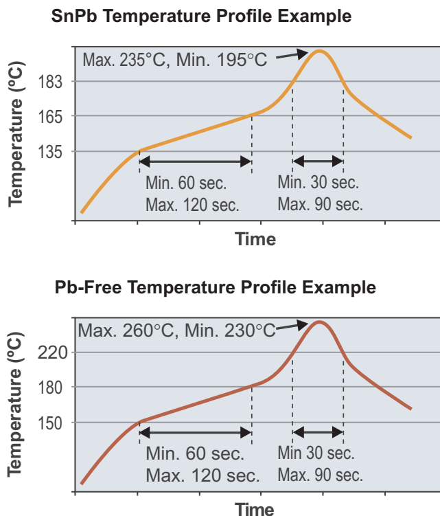
Figure 13. QFN/SOP Pb and Pb-Free Example Reflow Profiles
