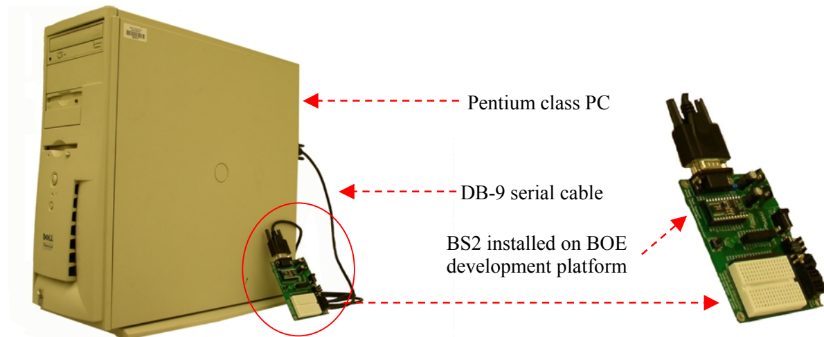
Figure 2: Hardware environment
