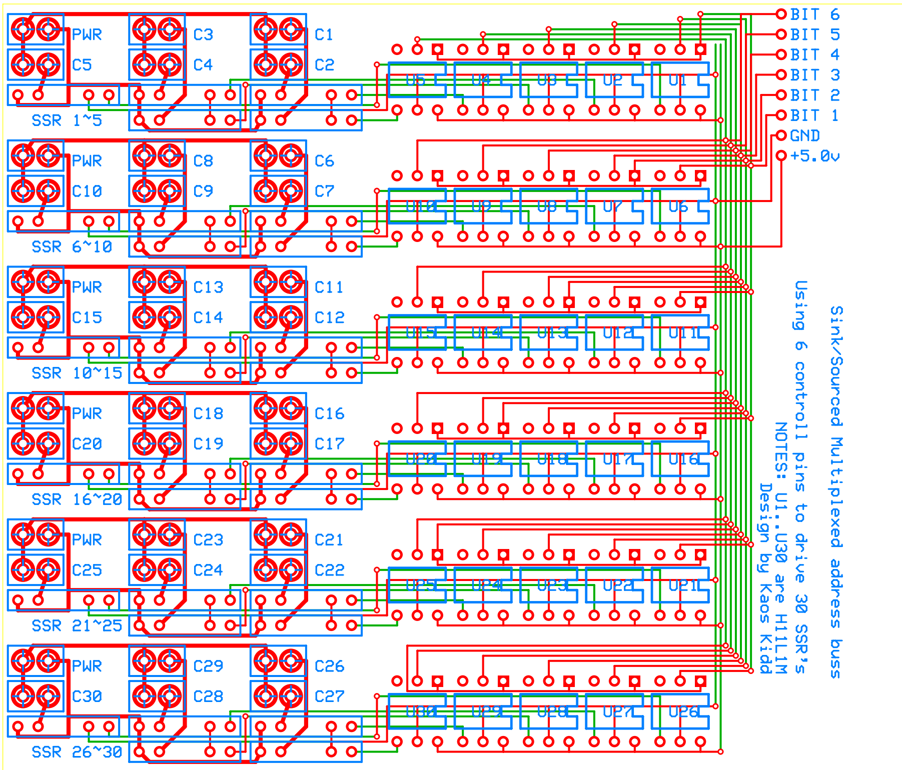
(Silkscreen, Top layer, Bottom layer)
