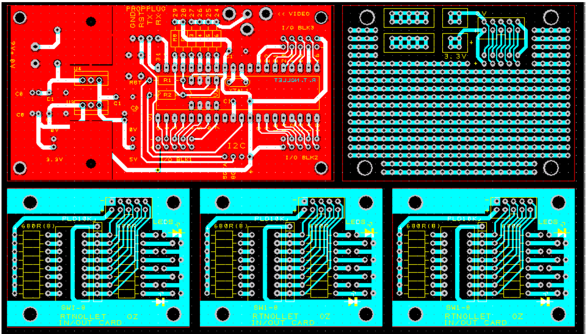
PropBus system Prelim 4/10/2007 R T Nollet
