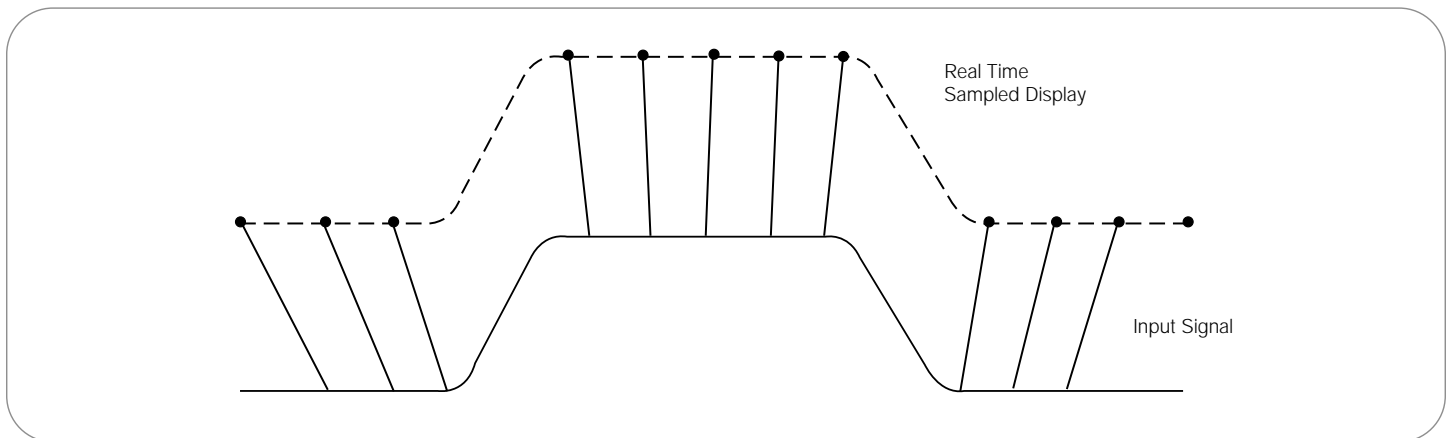
▶ Figure 30. In order to capture this 10 ns pulse in real-time, the sample rate must be high enough to accurately define the edges.
