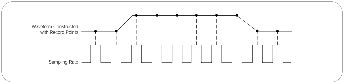
▶ Figure 29. Real-time sampling method.
