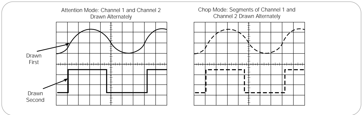
► Figure 24. Multi-channel display modes.
