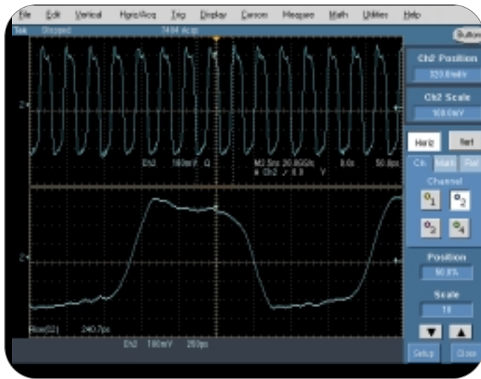
► Figure 48. Rise time characterization of a high-speed digital signal.
