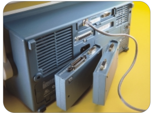
► Figure 55. A TDS3000 Series oscilloscope provides a wide array of communications interfaces, such as a standard Centronics port and optional Ethernet/RS-232, GPIB/RS-232, and VGA/RS-232 modules.
