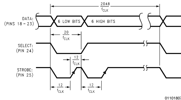
FIGURE 7. LM628 12-Bit DAC Output Multiplexed Timing
