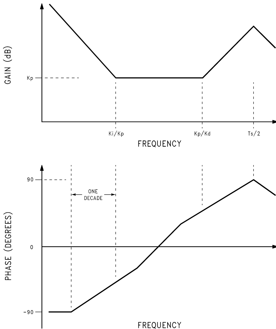
FIGURE 17. Bode Plots of PID Transfer Function
