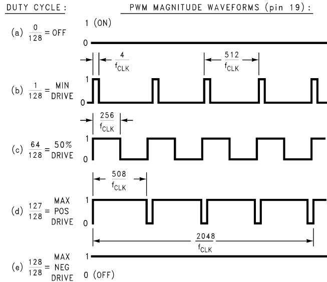
FIGURE 8. LM629 PWM Output Signal Format
