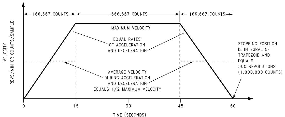
FIGURE 20. Trajectory Calculation Example Profile
