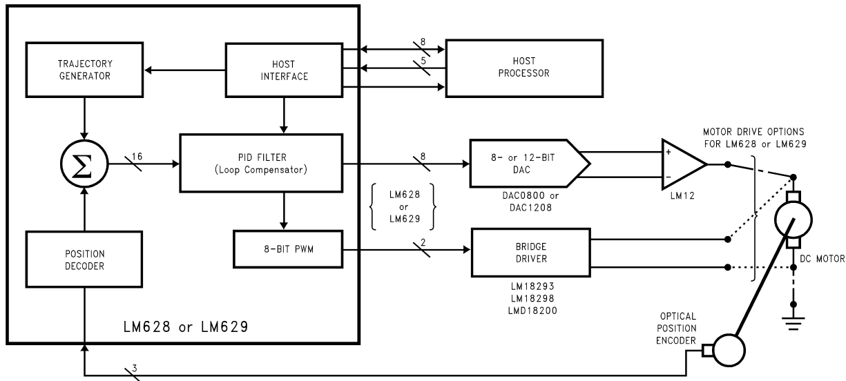
FIGURE 1. LM628 and LM629 Typical System Block Diagram
