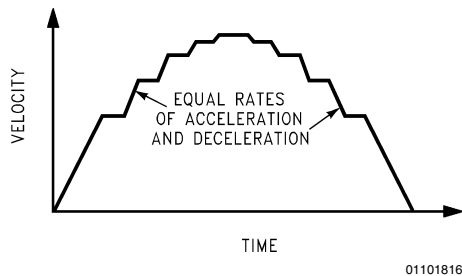
FIGURE 16. Generating a Non-Trapezoidal Profile
