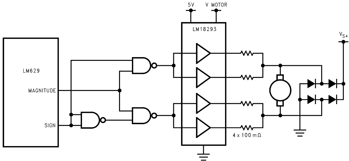
FIGURE 15. LM629 H-Bridge Motor Drive Example Using LM18293
