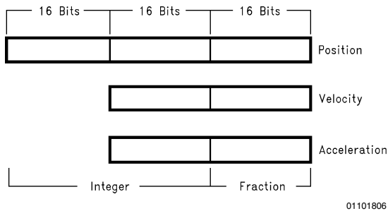
FIGURE 6. Position, Velocity and Acceleration Registers
