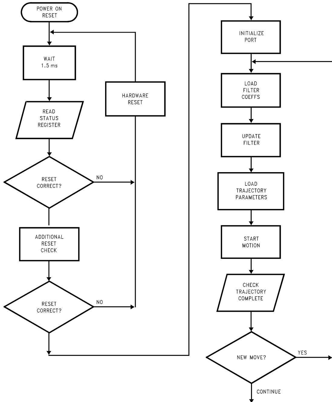
FIGURE 12. Basic Software Flow
