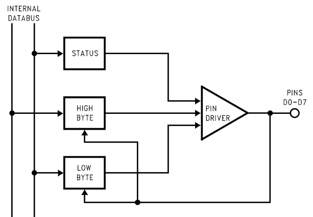
FIGURE 9. Host Interface Internal I/O Registers
