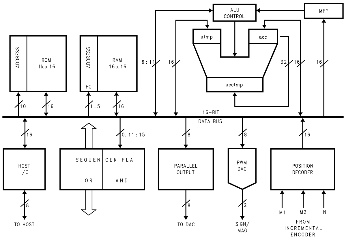
FIGURE 2. Hardware Architecture of LM628/629
