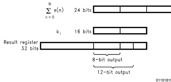
FIGURE 19. Scaling for k_i
