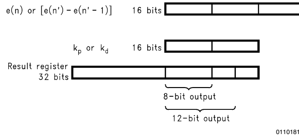
FIGURE 18. Scaling of k_p and k_d
