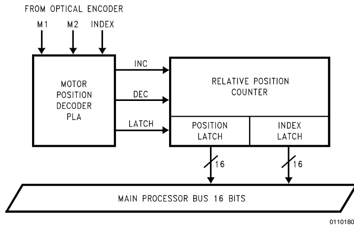
FIGURE 4. LM628/629 Motor Position Decoder
