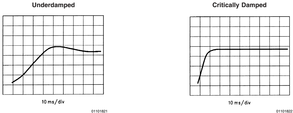
FIGURE 11. Position vs Time for 100 Count Step Input
