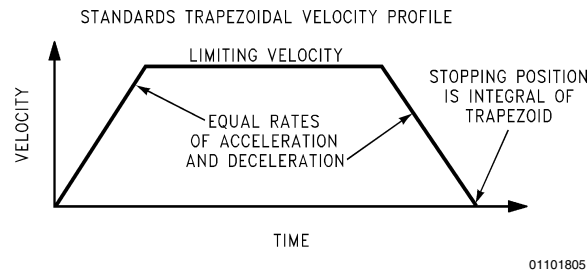
FIGURE 5. Typical Trajectory Velocity Profile
