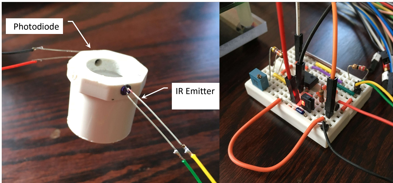
The original prototype break beam detector assembly and breadboard circuitry
