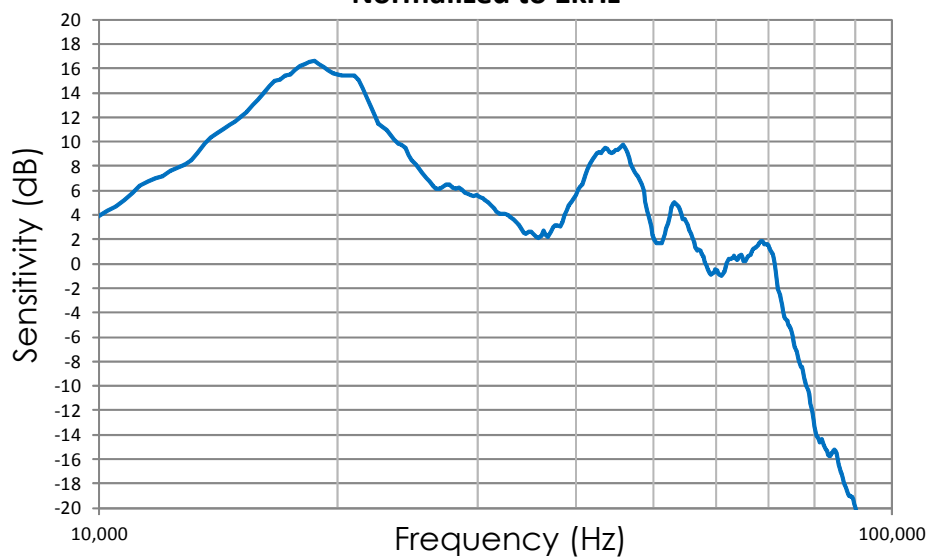
Typical Free Field Response Normalized to 1kHz
