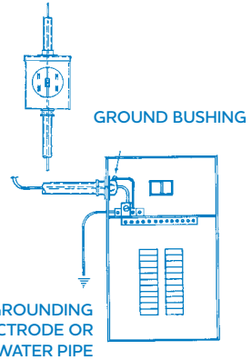
Backboard installation and panelboard mounting heights - Figure 11
