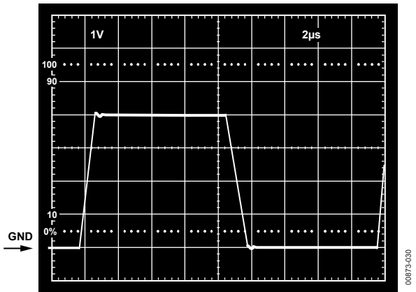
Figure 29. V_S = 5\text{ V} , 0\text{ V} ; Unity-Gain Follower Response to 0 V to 4 V Step
