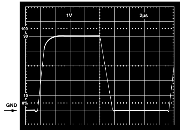
Figure 32. V_S = 5\text{ V} , 0\text{ V} ; Unity-Gain Follower Response to 0 V to 5 V Step
