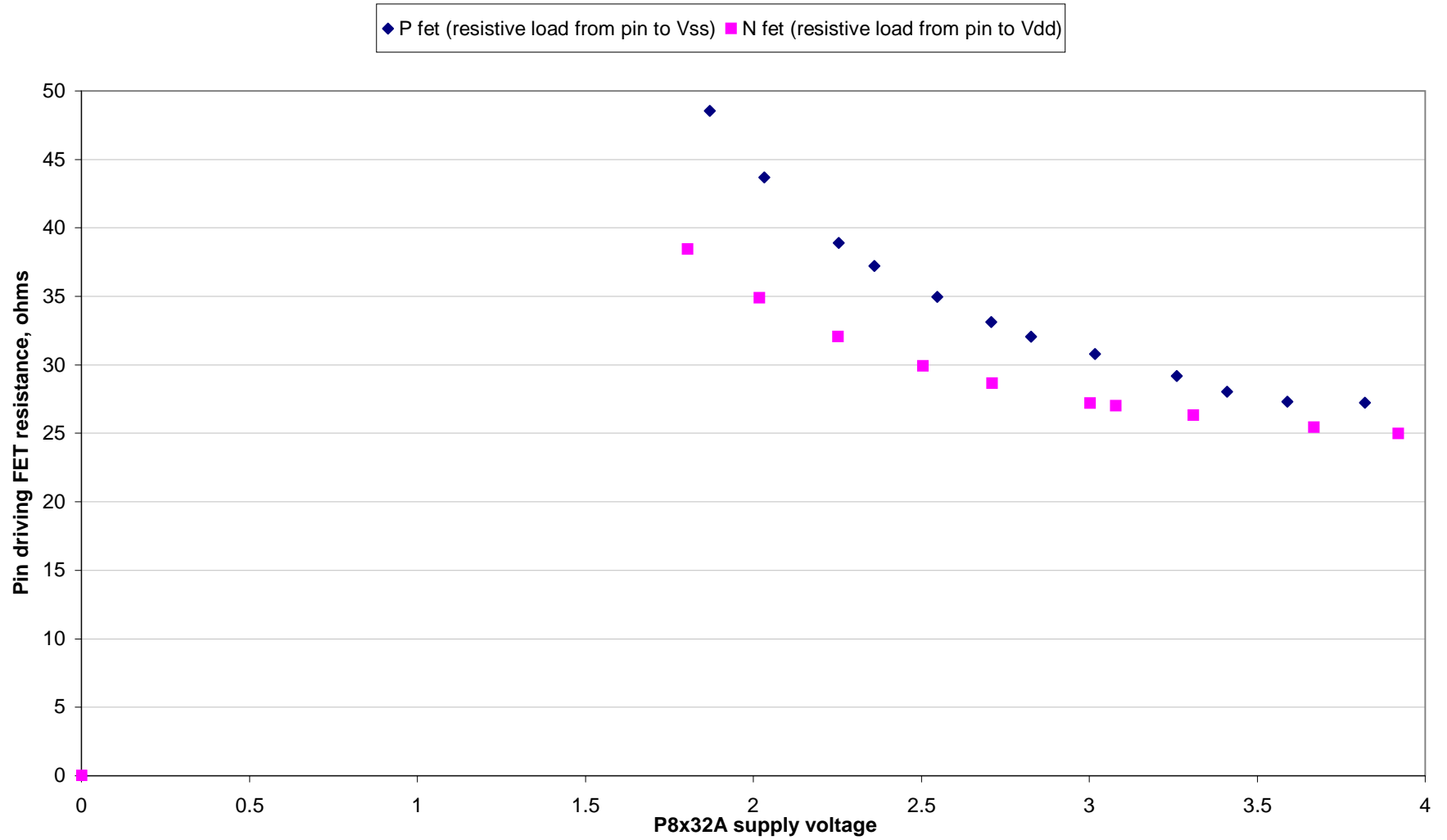
P8X32A: Pin driving FET resistance vs supply voltage, 270 ohm load
