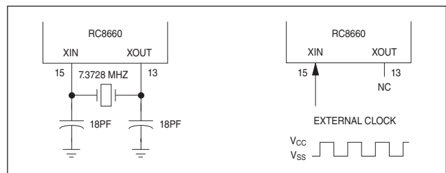
Figure 1. Clock Connections
