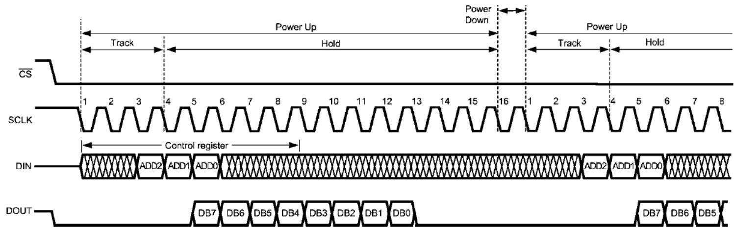
FIGURE 1. ADC088S052 Operational Timing Diagram
