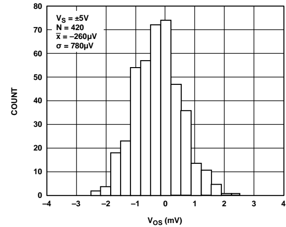
Figure 35. Input Offset Voltage Distribution
