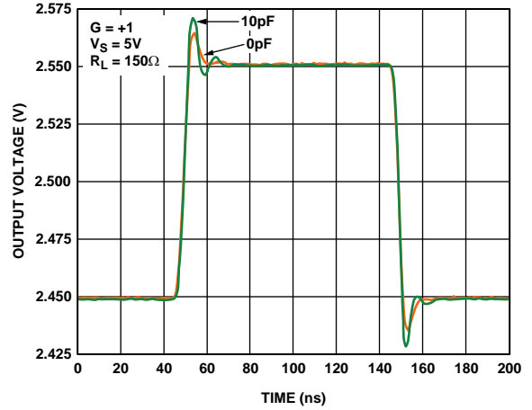
Figure 22. Small-Signal Transient Response for Various Capacitive Loads
