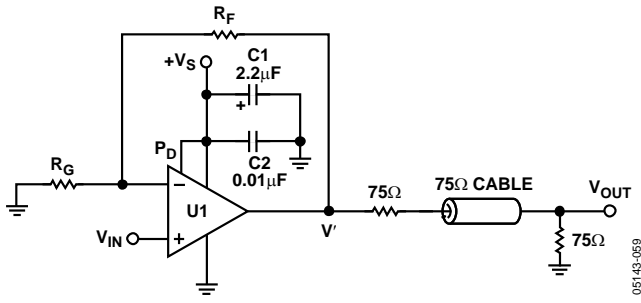
Figure 45. Video Amplifier
