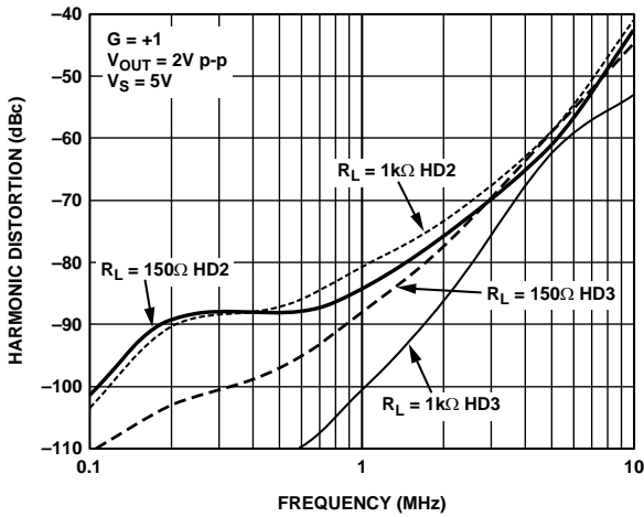
Figure 18. Harmonic Distortion vs. Frequency for Various Loads
