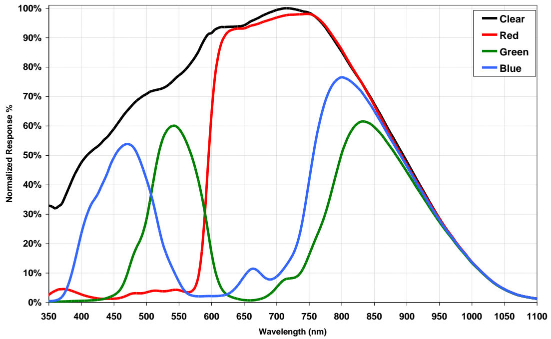
TCS230D Clear RGB Normalized Spectral Response to Clear @ 715nm
