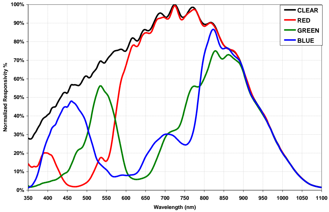
TCS230D Clear RGB Normalized Spectral Response to Clear @ 715nm
