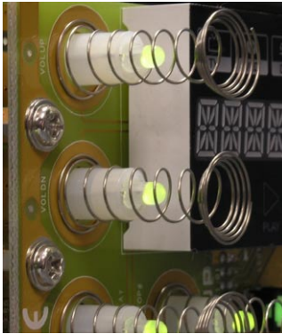
Fig. 5 - Asus S-presso uses Philipp™ springs attached to LED mounts to bridge the air gap to the panel and to simultaneously allow key backlighting.
