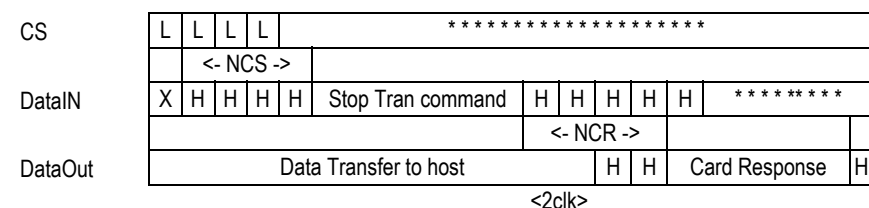
Figure 5-15. Multiple Block Read Timing
