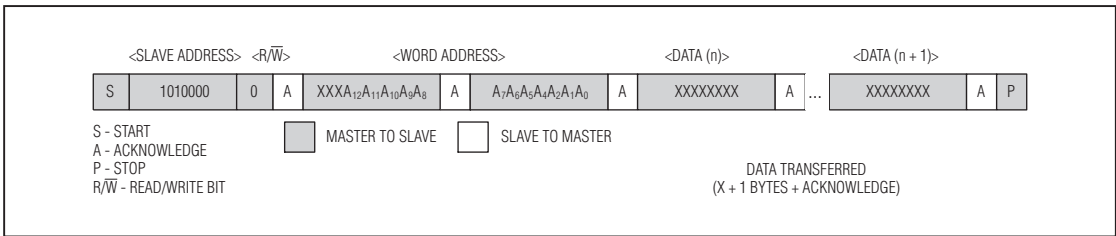
Figure 7. Data Write—DS32C35 FRAM Slave Receiver Mode
