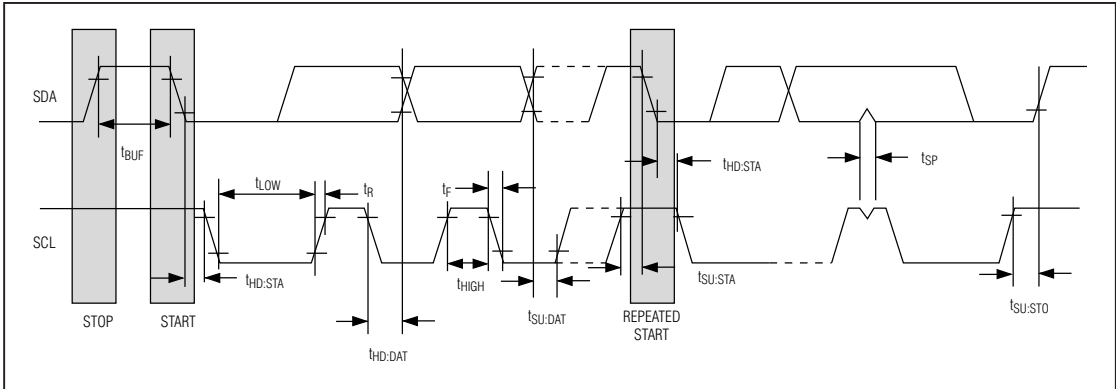
Figure 1. Data Transfer on I 2 C Serial Bus
