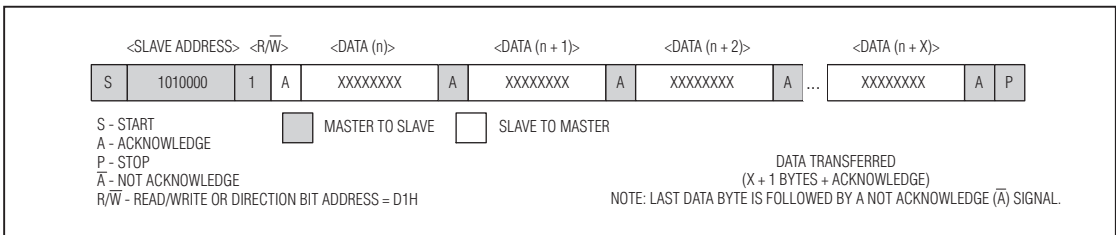
Figure 8. Data Read—DS32C35 FRAM Slave Transmitter Mode
