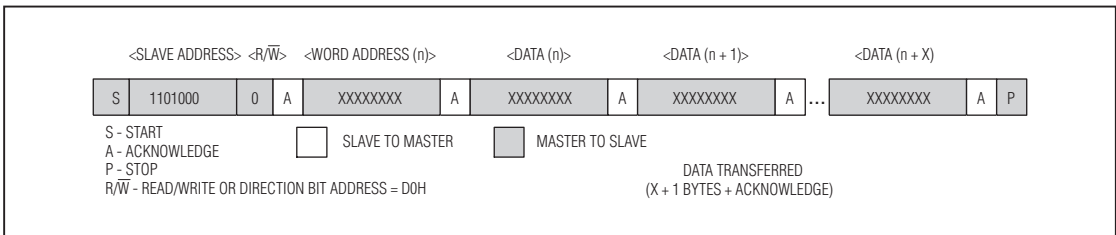
Figure 3. Data Write—RTC Slave Receiver Mode
