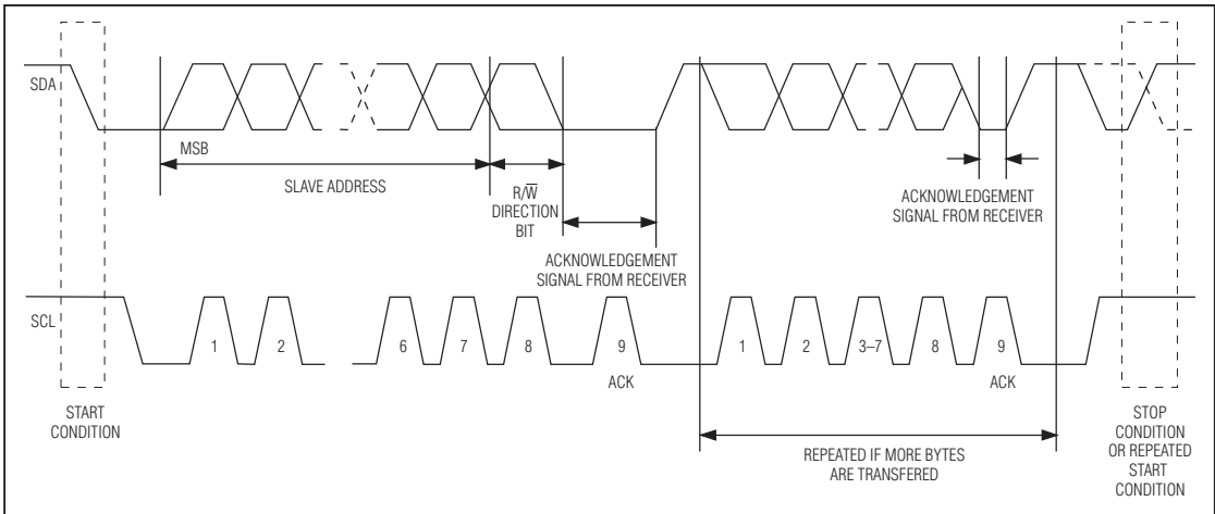
Figure 2. I 2 C Data Transfer Overview
