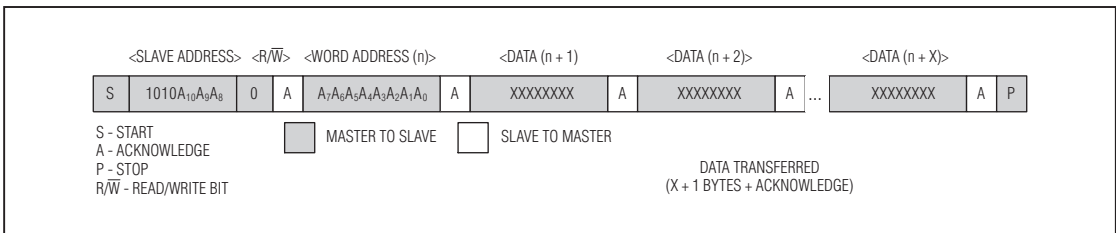
Figure 5. Data Write—DS32B35 FRAM Slave Receiver Mode
