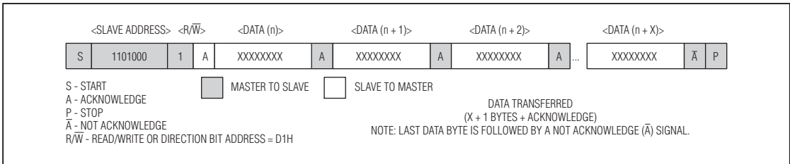
Figure 4. Data Read—RTC Slave Transmitter Mode
