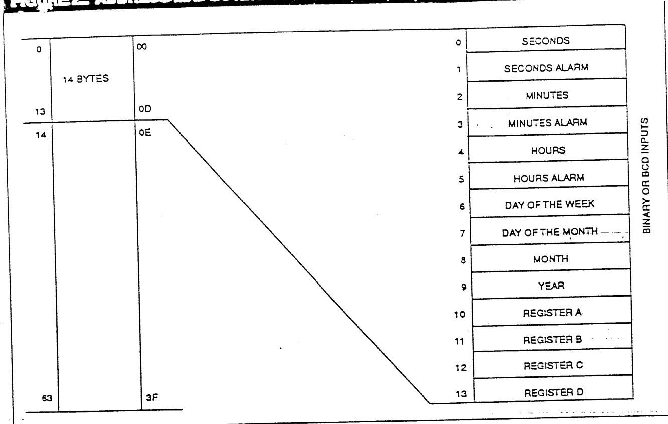
FIGURE 2 ADDRESS MAP DS1287
