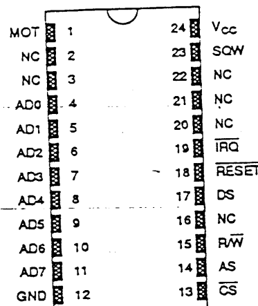
24 PIN ENCAPSULATED PACKAGE
