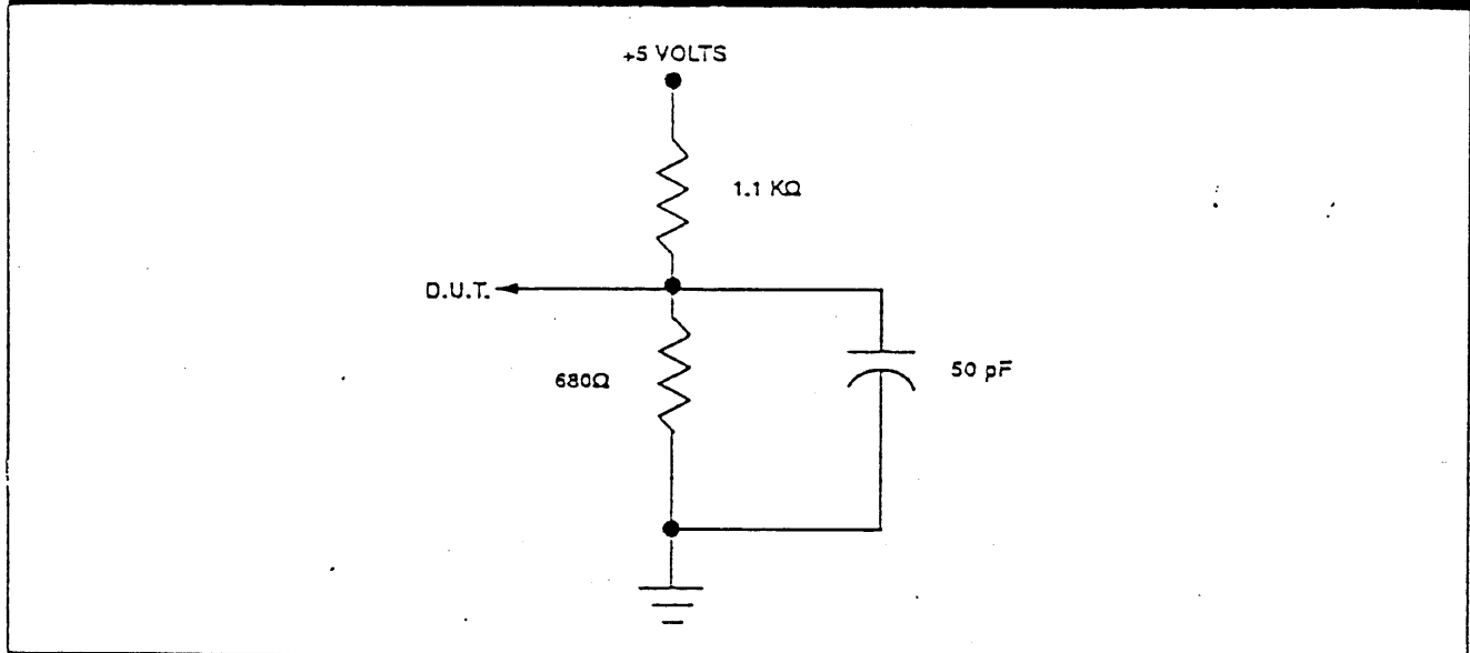
FIGURE 4: OUTPUT LOAD
