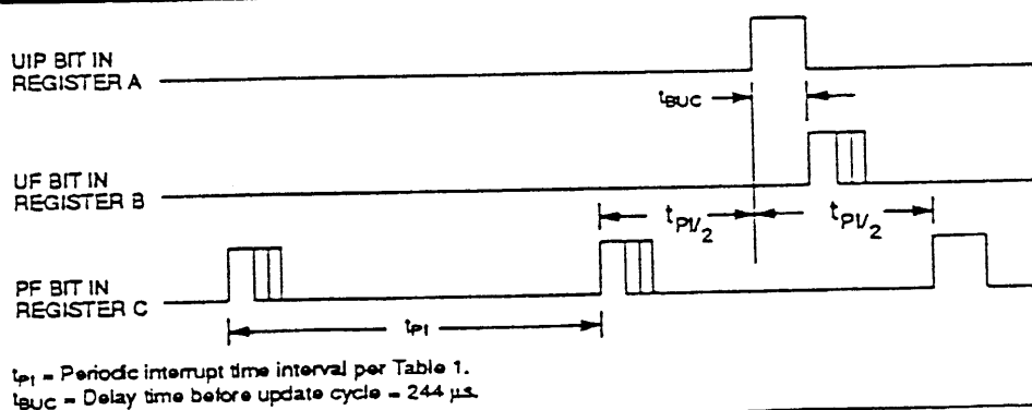
FIGURE 3: UPDATE-ENDED AND PERIODIC INTERRUPT RELATIONSHIP
