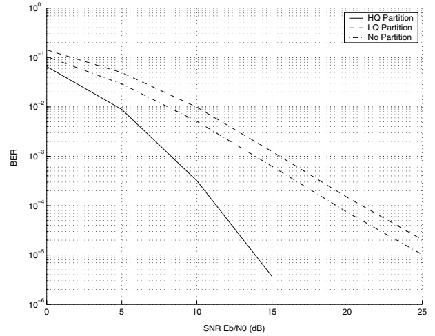
Fig. 7. Performance of different sub-channel partitions.
