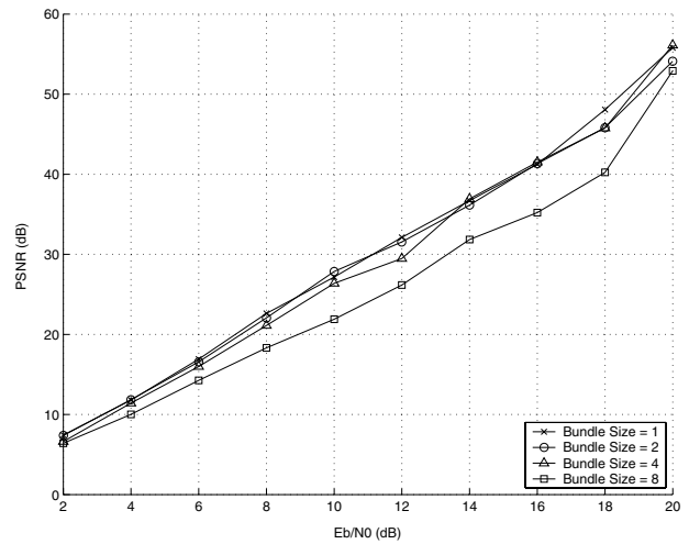
Fig. 12. PSNR performance for different sub-channel bundle sizes.
