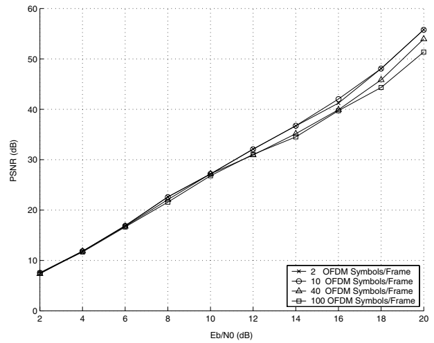
Fig. 11. PSNR performance for different frame sizes.
