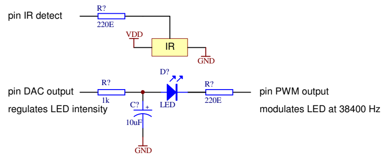
JBot obstacle detection circuit
