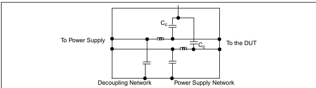
Figure 6. Coupling Network
