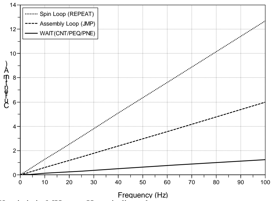
Typical Current of a Cog vs. Operating Frequency (Vdd = 3.3 V, Ta = 25° C)
