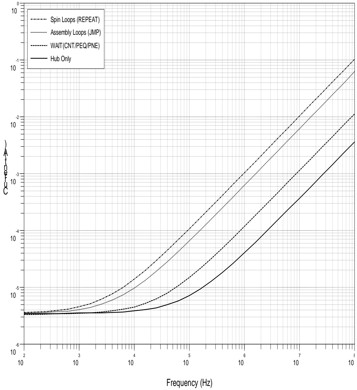
Typical Current Consumption of 8 cogs vs. Operating Frequency (3.3V, Ta = 25°C)
