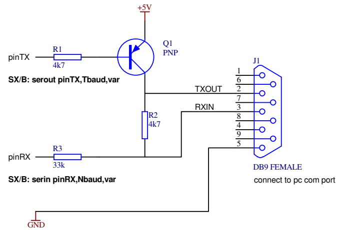
Half duplex serial I/O
