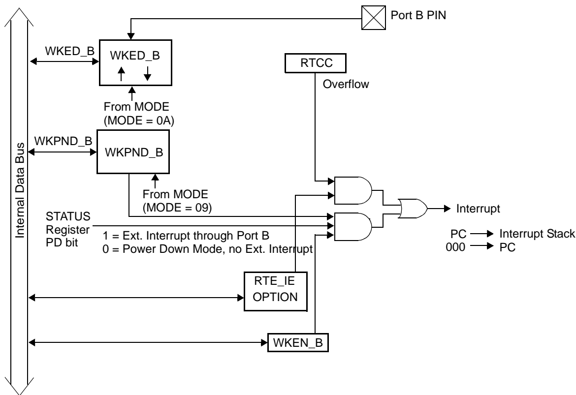
Figure 8-1. Interrupt Structure
