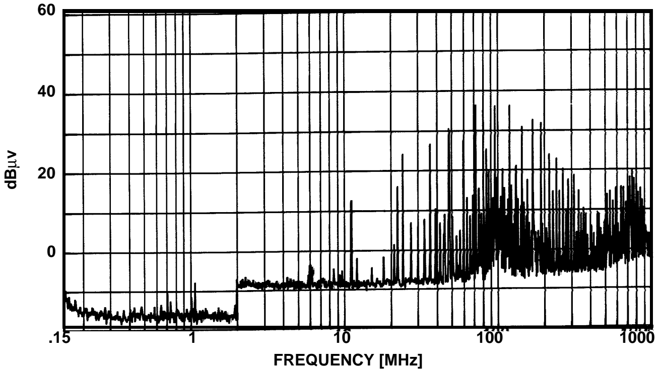
Figure 4. Emission Levels at Device Operating Frequency of 12 MHz - 28 SOIC
