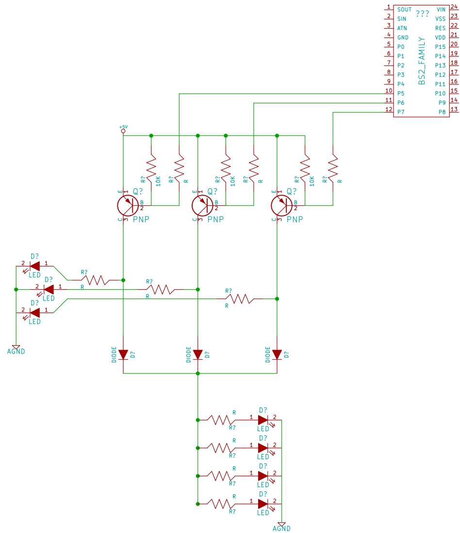
Final Version Components, discrete LEDs used in schematic
