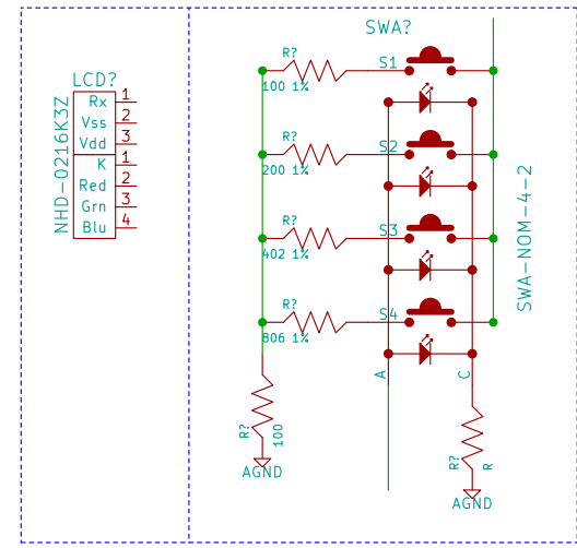
Final Version Components, discrete LEDs used in schematic
