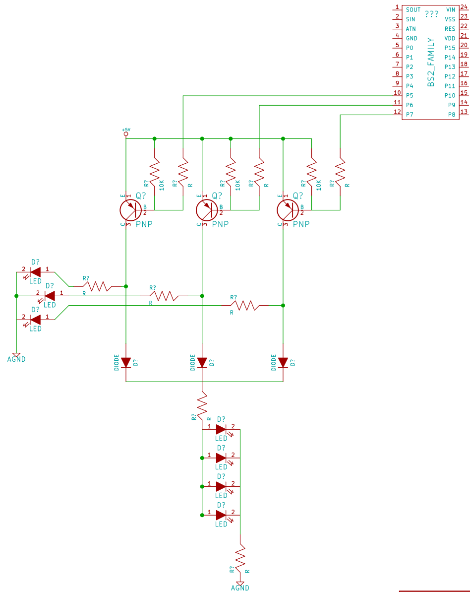
Final Version Components, discrete LEDs used in schematic
