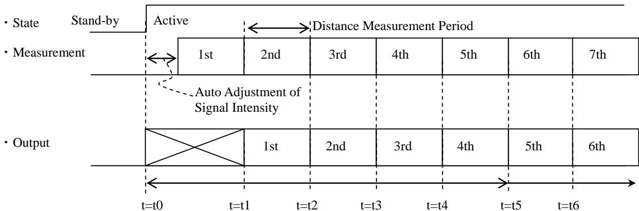
Fig.22 Median Filter
