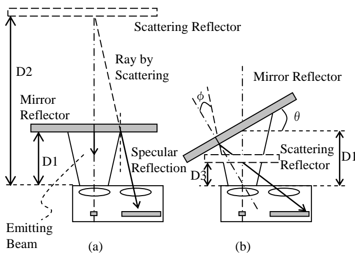
Fig.05 Mirror Reflector
