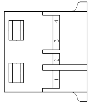
Wiring Diagram (Both Ends)
