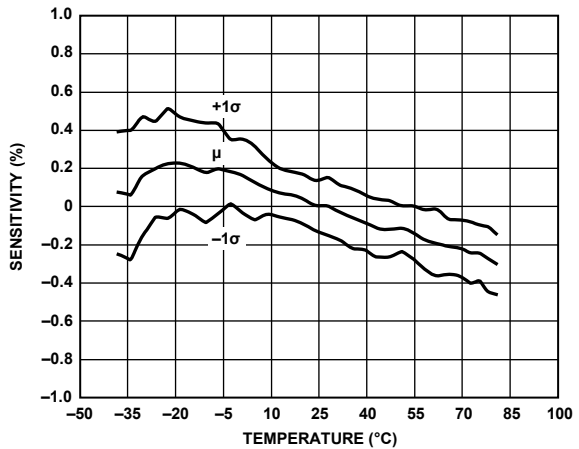
Figure 8. ADIS16350 Accelerometer Sensitivity vs. Temperature
