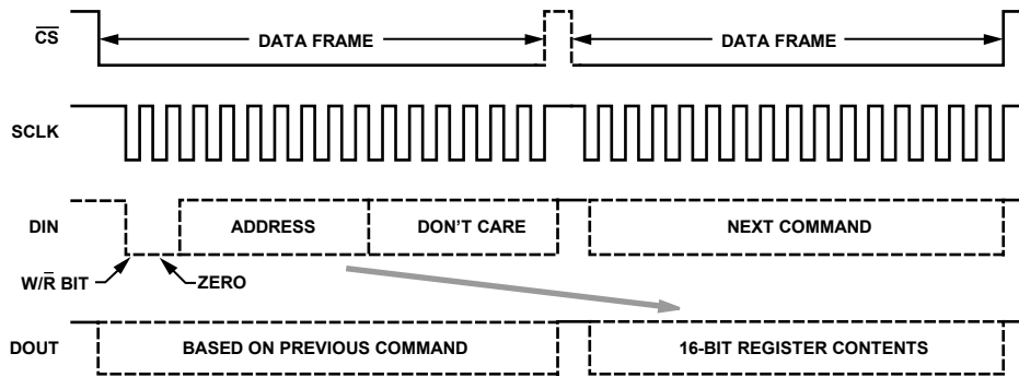
Figure 26. SPI Sequence for Read Commands
