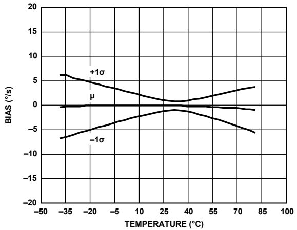
Figure 7. ADIS16350 Gyroscope Bias vs. Temperature
