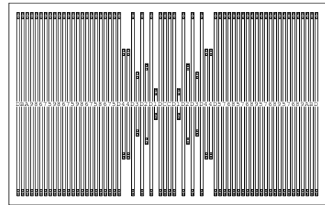
Matched resistor array layout
