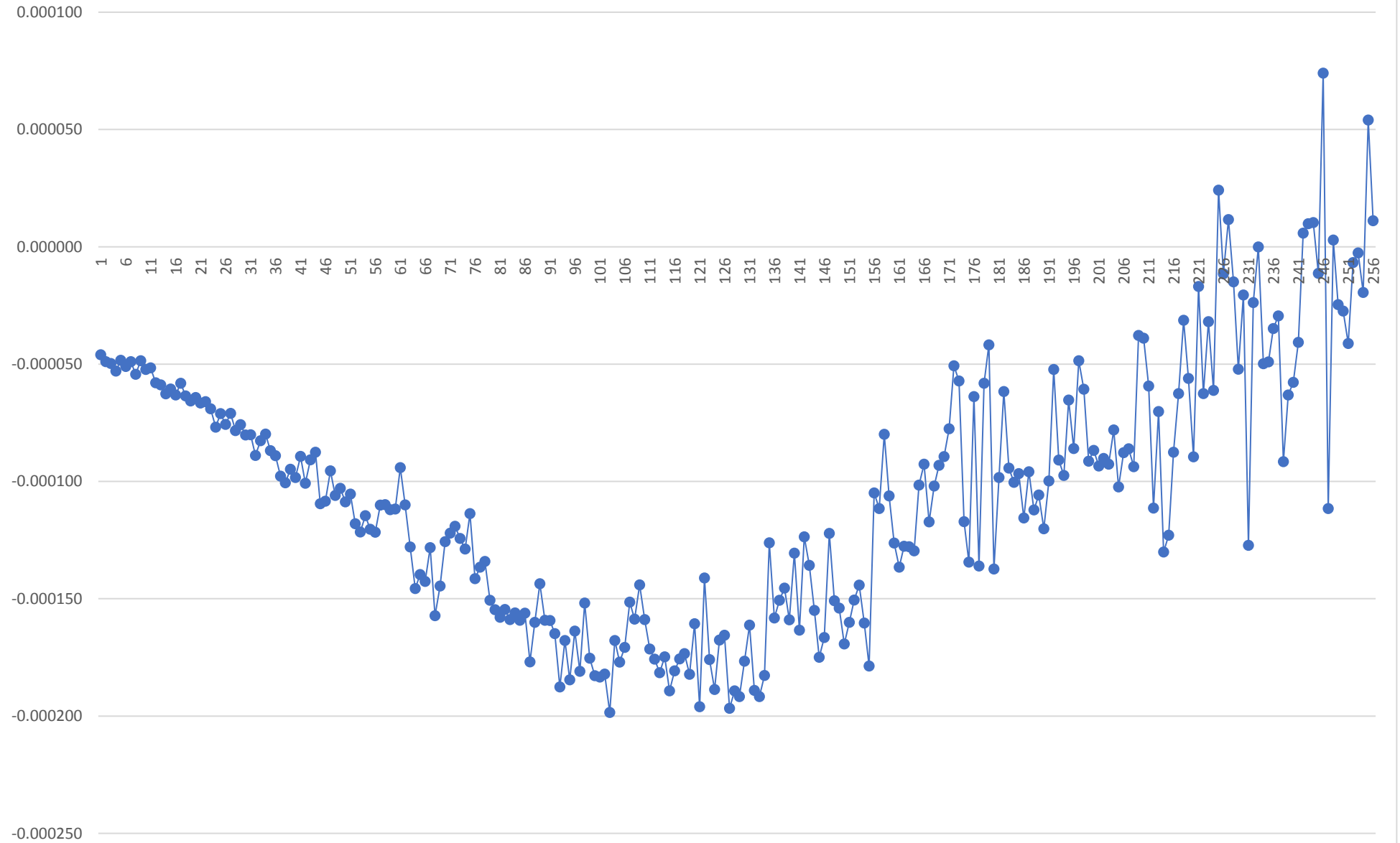
Board 2 Pin 0 DAC 2 (123R) Voltage on upramp vs downramp, by code
