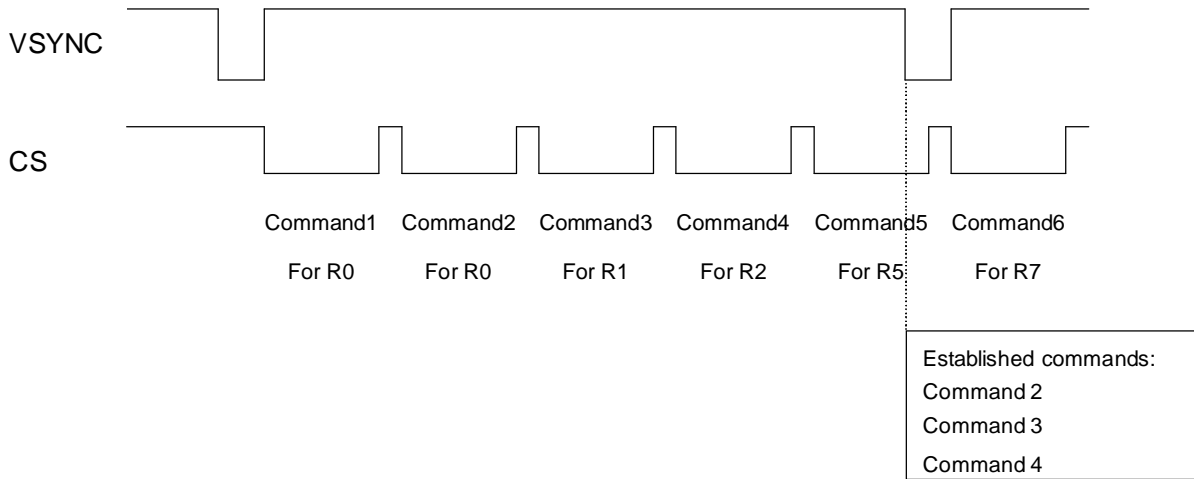
Fig. 8 Illustration of Serial Command Operation
