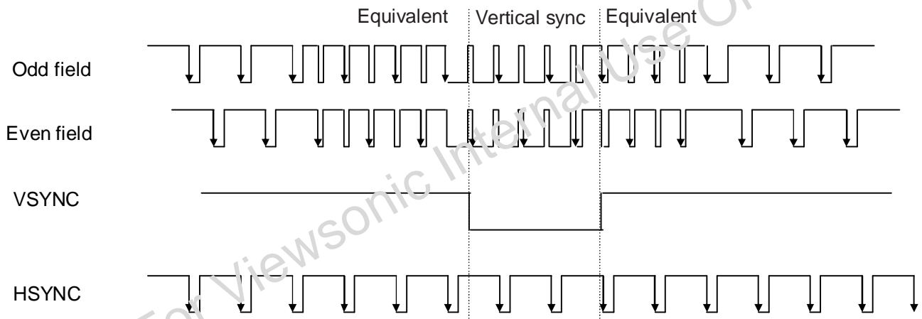
Fig. 6: CSYNC Data input format
