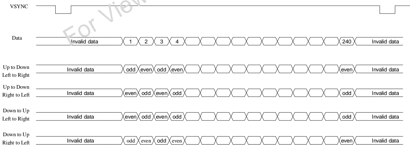
Fig 10. UPS051 even and odd lines definition
